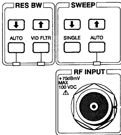
Figure 4-8: Resolution BW and Sweep Control
