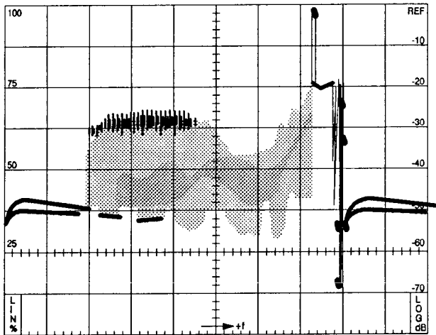
Figure 7-15: Video Field Using Internal or TV Field Triggering
