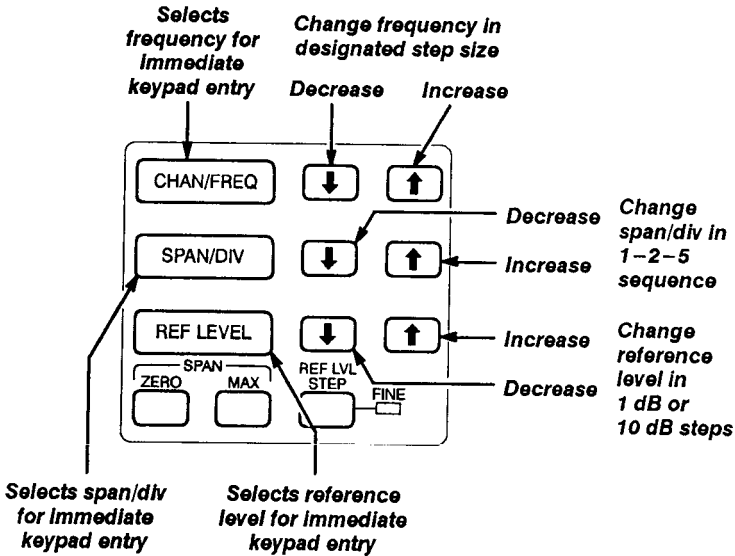
Figure 3-4: The Primary Controls
