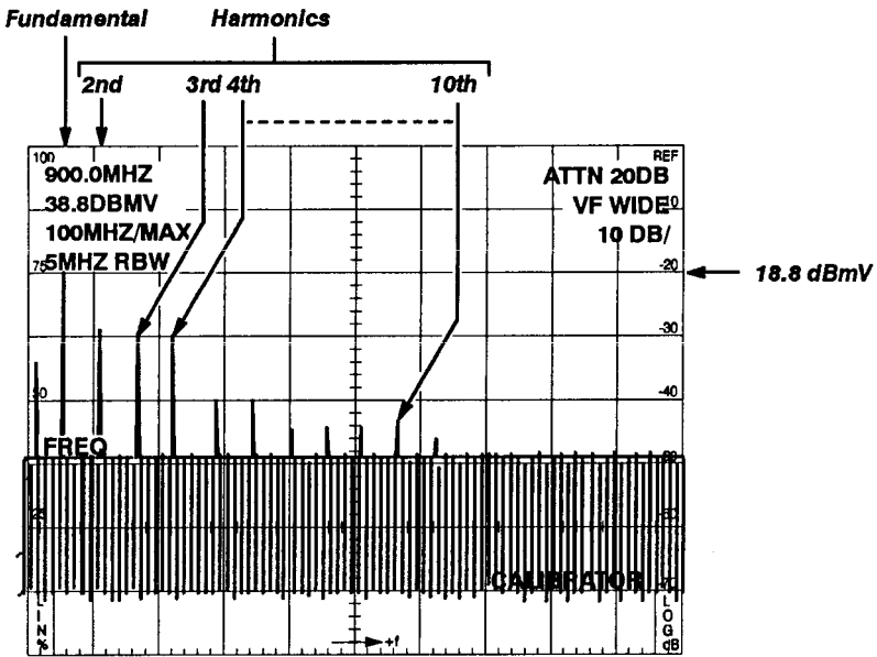
Figure 3-5: Callibrator Signal and Harmonics
